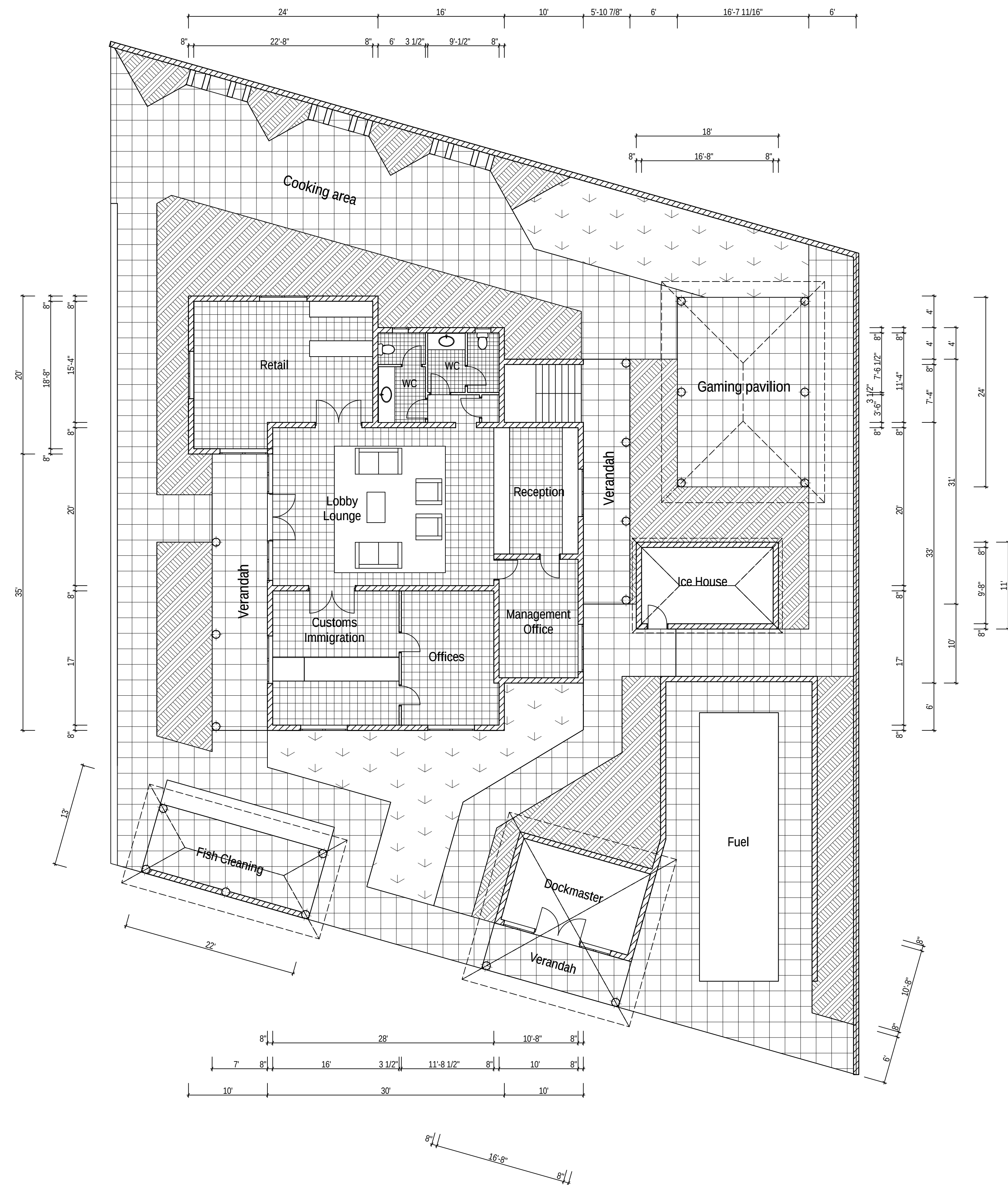
GROUND FLOOR
